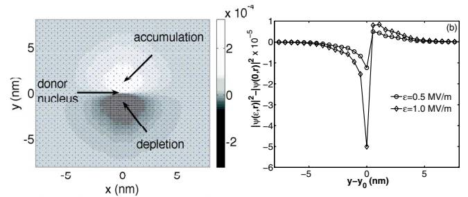
FIG. 2 (color online). (a) Electric field-induced differential map of donor electron wave probability density |\Psi(\epsilon, z_0)|^2 - |\Psi(0, z_0)|^2 shown as a 2D cut through the impurity center at z_0 = 16.29 \text{ nm} for \epsilon = 0.5 \text{ MV/m} . The electric field is directed along the negative y axis. (b) 1D cut through the center of the impurity showing the differential map of the probability density for two different electric fields.
