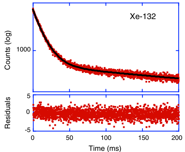
FIG. 2 (color online). Decay curve obtained with a proportional counter detector when injecting isotopically pure ^{132}\text{Xe} into SuperEBIT, and fit of two exponentials to the data. The decay curve of this isotope without hyperfine structure consists of a single-exponential radiative decay and a tail that represents electron capture by charge exchange with neutral residual gas. The fit residuals have been normalized to the signal; they show no discernible oscillation around the mean.
