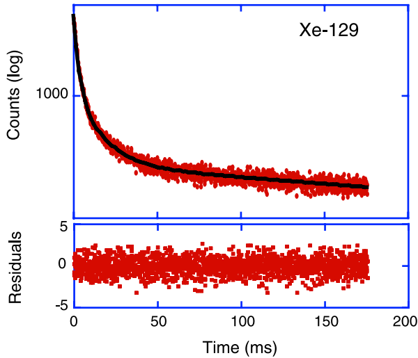
FIG. 3 (color online). Decay curve as in Fig. 2, but injecting isotopically pure ^{129}\text{Xe} into SuperEBIT, and a fit of three exponentials to the data. Evidently, the decay curve of this isotope with hyperfine structure is more complex than that of an isotope without HFS. The curve for ^{129}\text{Xe} has two major radiative decay components; isotopes of larger nuclear spin are expected to show even more components. The (normalized) fit residuals show no discernible oscillation around the mean.
