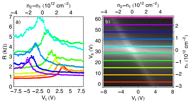
FIG. 2 (color online). (a) Resistance across the graphene sample at 4 K as a function of the top gate voltage for several back gate voltages, each denoted by a different color. (b) Two-dimensional gray scale plot of the same resistance as a function of both gate voltages. Traces in (a) are cuts along the correspondingly colored lines.
