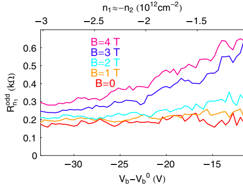
FIG. 5 (color online). Odd part of the resistance as a function of the back gate voltage V_b , with the constraint n_2 = -n_1 . Measurements were taken at 4 K for several values of the perpendicular magnetic field B .
