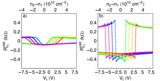
FIG. 4 (color online). (a) Using the strongly diffusive model described in the text, one can predict the resistance as a function of the top gate voltage V_t for several values of the density n_1 (each represented by the same color as in Fig. 3). Here we plot the odd part of this calculated resistance (cf. Fig. 3) for a barrier smoothness d = 40 nm and a width w = 1.7 \text{ }\mu\text{m} . (b) Similar curves for several densities n_1 using the ballistic model described in the text. The curves are plotted only for densities n_2 not too close to zero: n_2 > 10^{11} \text{ cm}^{-2} (the model diverges at n_2 = 0 ) and dashed lines link the curves at opposite sides of n_2 = 0 .
