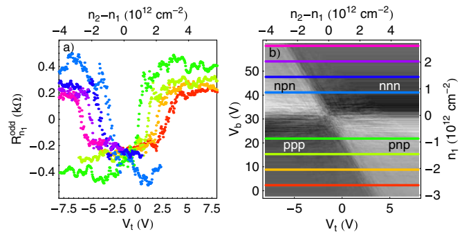
FIG. 3 (color online). (a) Odd component of the resistance: the part which depends on the sign of the density n_2 in region 2. (b) Gray scale plot of the odd component of the resistance for many values of n_1 . Colored lines are the cuts shown in (a).
