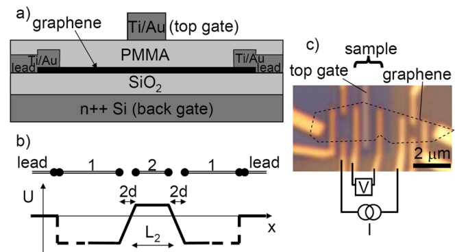
FIG. 1 (color online). (a) Cross-section view of the top gate device. (b) Simplified model for the electrochemical potential U of electrons in graphene along the cross section of (a). The potential is shifted in region 2 by the top gate voltage and shifted in both regions 1 and 2 by the back gate voltage. (c) Optical image of the device. The barely visible graphene is outlined with a dashed line and the PMMA layer appears as a (blue) shadow. A schematic of the four-terminal measurement setup used throughout the Letter is shown.
