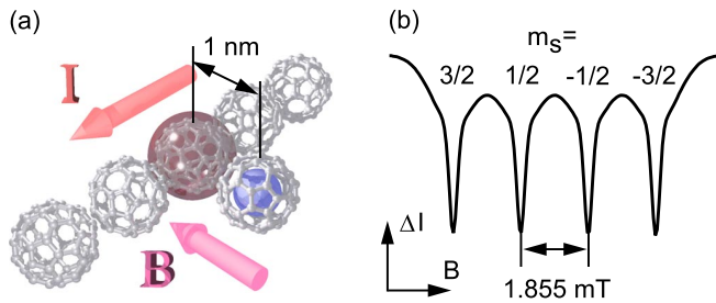
FIG. 3 (color online). (a) Schematic illustration of an electrical readout of a N@C 60 endohedral fullerene spin. The localized spin involved in spin-dependent transitions, marked by a surrounding sphere, is dipolarly coupled to the adjacent N@C 60 spin. (b) The expected spectrum for 52 MHz strong coupling of the S = \frac{3}{2} N@C 60 spin to an S = \frac{1}{2} state in C 60 .
