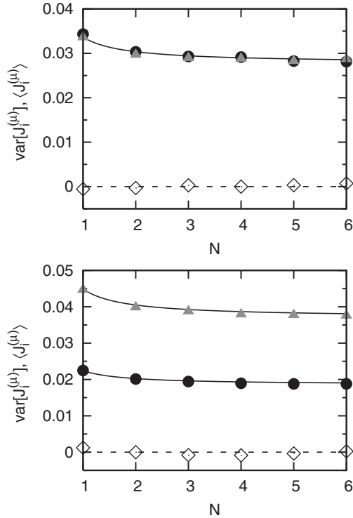
FIG. 2. Average and variance of the transverse spin current vs the number of modes. Top panel: longitudinally symmetric configuration with N_1 = N_2 = 2N_3 = 2N_4 = 2N ; bottom panel: longitudinally asymmetric configuration with N_2 = N_4 = 2N_1 = 2N_3 = 2N . In both cases the total number of modes N_T = 6N . The solid (dashed) lines give the analytical prediction (9) and (11) for the mean (variance) of the spin currents. Empty diamonds correspond to \langle J_i^{(\mu)} \rangle , circles to \text{var}[J_3^{(\mu)}] and triangles to \text{var}[J_4^{(\mu)}] .
