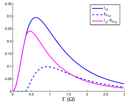
FIG. 2 (color online). SR phenomena quantified in terms of information-theoretic measures for a systems of two coupled and weakly driven spins ( J/\Omega = 1.5 ) at a zero temperature. Presented results are for \delta = 0 but deviations up to \delta/\Omega \sim 10^{-2} yield very small deviations from the exact resonance behavior.
