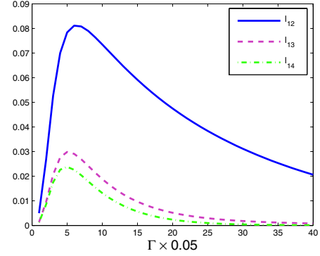
FIG. 3 (color online). System's response for a chain of N = 4 qubits at T = 0 with J_i/\Omega_i = 1.5 , ( i = 1 \dots 4 ) as quantified by an information-theoretic measure, the quantum mutual information. Under the evolution given by H_{\text{eff}} , entanglement is restricted to nearest neighbors only and E_{F_{13}} = E_{F_{14}} = 0 .
