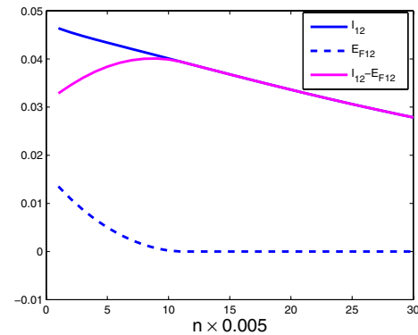
FIG. 4 (color online). Information-theoretic measures as a function of the bath's mean boson number (temperature) for a chain of N = 4 spin with J_i/\Omega_i = 1.5 and \Gamma_i/\Omega_i = 1 , i = 1 \dots 4 .
