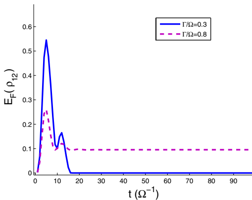
FIG. 1 (color online). Entanglement time evolution for two weakly driven qubits with longitudinal coupling of strength J/\Omega = 1.5 at T = 0 . If the noise strength \Gamma is sufficiently large, the system is inseparable in the steady state (pink dashed line).
