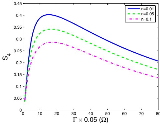
FIG. 5 (color online). System's response for a chain of N = 4 qubits with J/\Omega = 1.5 as quantified by S_4 = \langle \sum_{i=1}^4 \sigma_x^i / 4 \rangle as a function of the noise strength \Gamma and for different values of the external temperature.
