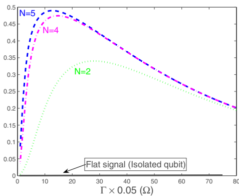
FIG. 6 (color online). Single qubit steady-state response for weakly driven arrays of 2, 4, and 5 qubits with J/\Omega = 1.5 and \bar{n} = 0.01 . The zero signal corresponds to a resonantly driven uncoupled oscillator. Interqubit coupling yields an enhanced response as a function of the number N of oscillators in the array.
