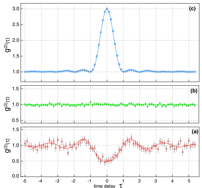
FIG. 3 (color online). Experimental measurement of g^{(2)}(\tau) with normalized time delay \tau in units of bandwidth \pi/\Omega = 8.3 \mu\text{s} . (a) displaced-squeezed state, (b) coherent state, (c) -biased-thermal state, curves are theoretical predictions.
