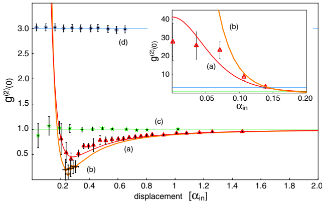
FIG. 4 (color online). Experimental measurement of g^{(2)}(0) as a function of displacement \alpha_{in} . (a) displaced- squeezed state, (b) weak displaced-squeezed state, (c) coherent state, (d) biased-thermal state, curves are theoretical predictions.
