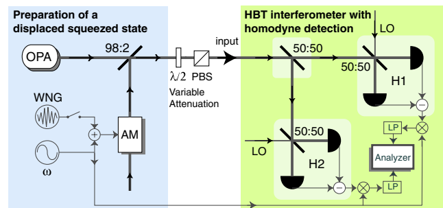
FIG. 1 (color online). Schematic of the experimental setup. OPA optical parametric amplifier, \lambda/2 half-wave plate, PBS polarizing beam splitter, x:y beam splitter with transmission x , H1/H2 homodyne detectors, AM amplitude modulator, \omega function generator, WNG white-noise generator, \otimes mixer, LP low-pass filter.
