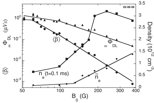
FIG. 3. Measured m\Phi_{DL} , \langle\beta\rangle , \bar{n}_e , and \bar{n}_e^m vs B_0 . Pulse duration t = 2 ms, \max P_{rf} = 9.6 kW, f_s = 13.967 MHz, P_{H_2} = 1.08 mTorr, B_M = 2800 – 5000 G.
