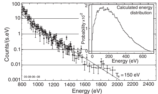
FIG. 4. Measured x-ray spectrum: mP_{rf} = 9.6 kW; m\bar{n}_e = 1.6 \times 10^{12} \text{cm}^{-3} ; m\Phi_{DL} = 5 \mu\text{Vs} ; f_s = 14.000 MHz (no FM); P_{H_2} = 1.09 mTorr; B_0 = 56 G; B_M = 2900 G, where subscript m means maximum value. The spectrum shape is fit by T_e = 150 eV. Inset: electron energy distribution calculated with the RMF code.
