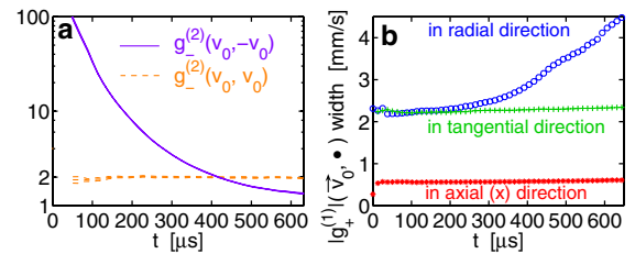
FIG. 3 (color online). Evolution of correlations between scattered atoms. Parameters and \vec{v}_0 as in Fig. 2. (b): The full-width half-maximum (FWHM) width of |g_{\pm}^{(1)}| in velocity space.
