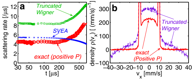
FIG. 4 (color online). Comparison of exact and approximate methods. Panel (a): Rate of scattering out of coherent wave packets. Obtained by counting atoms outside of spheroidal regions covering the coherent wave packets centered at \pm v_Q and \pm 3v_Q . Panel (b): Distribution of axial ( x ) velocity of scattered atoms at t = 657 \mu\text{s} ; In both panels: S = 2048 (Pos. P), S = 672 (Wigner).
