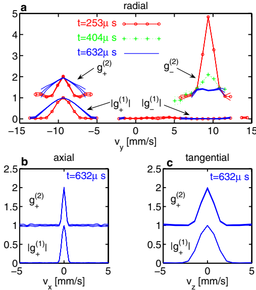
FIG. 2 (color online). Correlations between scattered atoms. All are between scattered atoms at a maximum density point in the shell (with velocity \vec{v}_0 = (0, -9.37, 0) mm/s relative to the COM) and those with a shifted velocity \vec{v} , where: (a): \vec{v} = (0, v_y, 0) , (b): \vec{v} = (v_x, 0, 0) , and (c): \vec{v} = (0, 0, v_z) . To reduce statistical noise, averages g_{\pm}^{(n)} = \frac{1}{V_0} \int g^{(n)}(\vec{v}_0 + \delta\vec{v}, \vec{v} \pm \delta\vec{v}) d^2\delta\vec{v} , over a small local volume V_0 in velocity space are plotted. Triple lines are 1\sigma errors.
