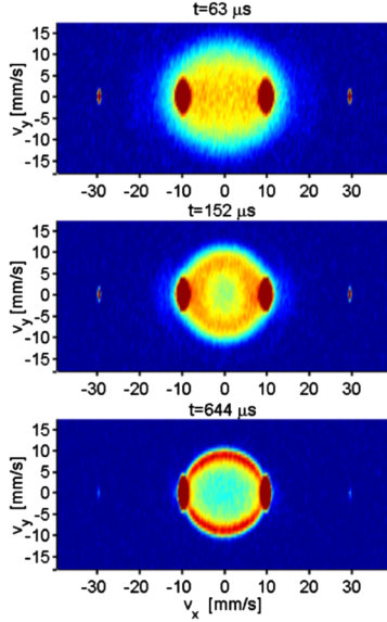
FIG. 1 (color online). Evolution of velocity distribution. The distribution \rho(v_x, v_y) has been integrated over one transverse dimension z . Shading indicates differing density (its range varies between panels). S = 2048 trajectories.
