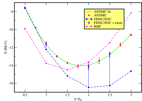
FIG. 1 (color online). Equation of state of symmetric nuclear matter calculated with different methods. Red circles represent AFDMC results with statistical error bars and the green line is the fitted functional form described in the text. Dashed lines correspond to calculations performed with other methods [19] (blue line with squares: FHNC-SOC; magenta with diamonds: BHF). Blue triangles represent the FHNC-SOC energies corrected by including the low order of elementary diagrams as described in the text. Blue arrows show the corresponding energy shift, which increases at higher densities.
