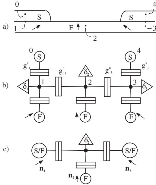
FIG. 1. Building up the circuit-theory model. (a) S/F/S structure exhibiting TPE [7]. (b) The corresponding circuit consists of three nodes representing parts 1–3 of the structure. (c) Nodes 1 and 3 are replaced by effective S/F reservoirs.
