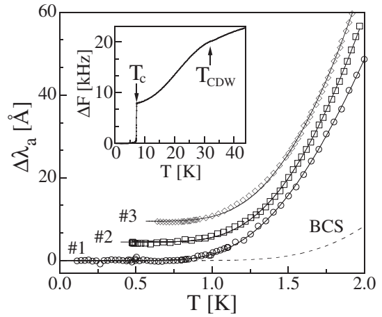
FIG. 1. Temperature dependence of the in-plane penetration depth, \Delta\lambda_a in single crystals of NbSe 2 . Data for three different samples are shown, offset for clarity. The absolute scale of \Delta\lambda_a is most accurate for sample 1 (see text). For sample 2 the data have been divided by 1.3. Inset: Frequency shifts at higher temperature showing the charge density wave transition.
