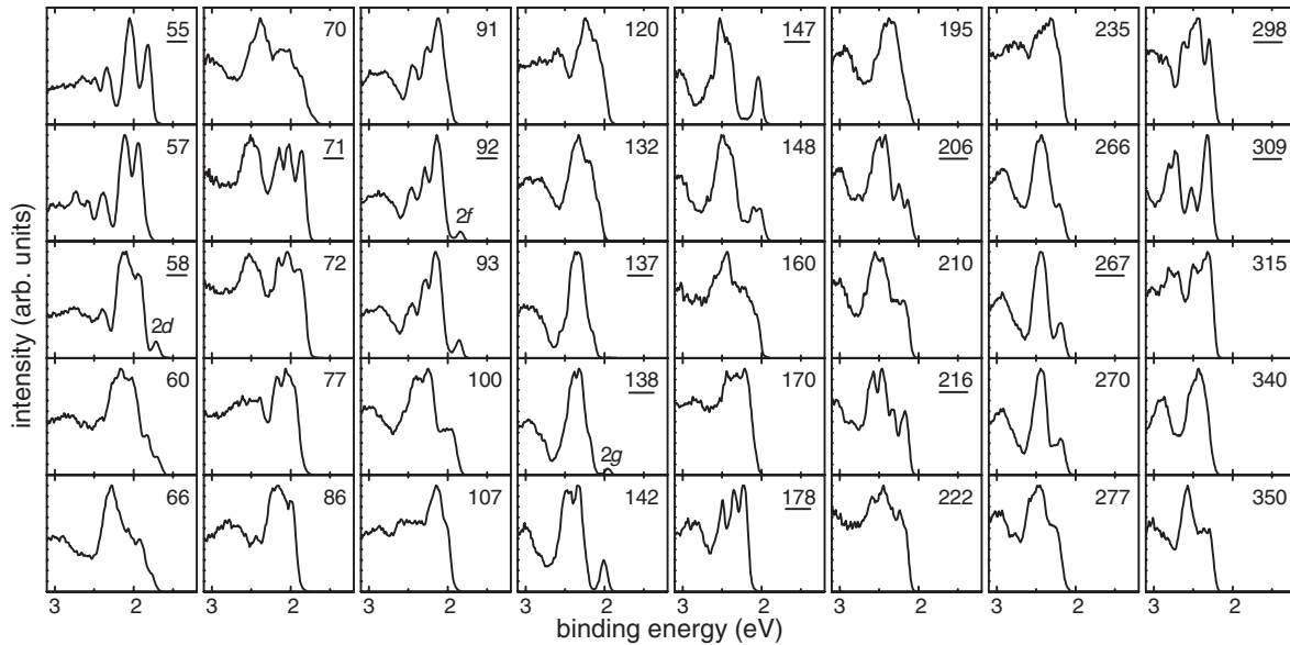
FIG. 1. Photoelectron spectra of cold ( T \approx 100 K) sodium cluster anions \text{Na}_n^- ( n = 55\text{--}350 ), measured at a photon energy of 4.02 eV. Underlined numbers indicate sizes with prominent features.
