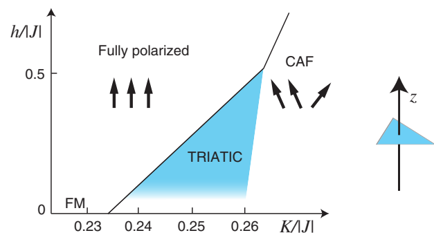
FIG. 1 (color online). (Left) Schematic phase diagram for the spin-1/2 J - K multiple spin exchange model on a triangular lattice in applied magnetic field, in the parameter range where J < 0 is FM and K \geq 0 is AF. A triatic phase with magnetic octupolar order appears in the shaded region between fully polarized and canted AF (CAF) phases. (Right) Schematic spin structure of this triatic order, which is invariant under spin rotations of 2\pi/3 about the z axis.
