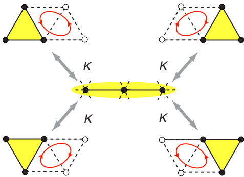
FIG. 2 (color online). The four-spin cyclic exchange operator can be used to propagate three flipped spins (●) in a polarized FM background by tunneling between compact triangular and straight line configurations.
