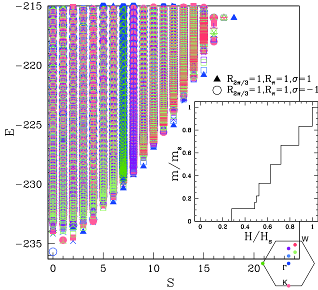
FIG. 4 (color online). Energy spectrum of the J - K model for N = 36 spin cluster with J = -4 and K = 1 , showing the oscillation in energies of the lowest lying states in spin sectors in the period three for large S . The inset shows the magnetization process m/m_s . Jumps of |\Delta m| = 3 , corresponding to octupolar order, are clearly visible at large H .
