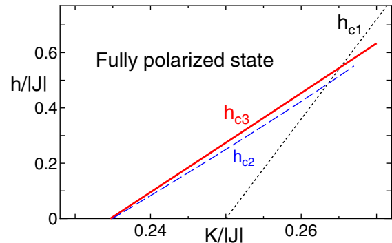
FIG. 3 (color online). Critical fields h_{c1} (dotted line), h_{c2} (dashed line), and h_{c3} (solid line), where one-, two-, and three-magnon instabilities destabilize the fully polarized state in the J - K model with FM J < 0 . The lines of h_{c1} and h_{c2} are given from exact solutions. The variationally estimated line h_{c3} gives an exact lower bound for three-magnon instability line.
