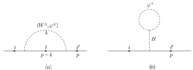
FIG. 1. Fermion mixing self-energy diagrams. H and \phi^\pm denote Higgs and charged Goldstone bosons, respectively. Diagram (b) is included to cancel the gauge dependence in the diagonal contribution of diagrams (a).
