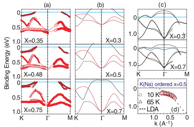
FIG. 3 (color online). Experiment versus theory: Comparison of (a) experimental band structures for x = 0.35 , x = 0.48 , and x = 0.75 with (b) LDA + large- U calculation [17] and (c) LAPW calculations [14]. (d) For sodium- or potassium-ordered samples, x = 1/2 , the e'_g band is always below the Fermi level ( \sim 250 meV) at the temperature below or above insulating transition points.
