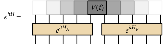
FIG. 1 (color online). Decomposing the propagator: for a given time t the propagator e^{itH} may be written as a product of e^{it(H_A+H_B)} and V(t) , where H_A ( H_B ) is the Hamiltonian with interaction terms only between spins in region A (between spins in region B ) and V(t) is a unitary operator which ‘‘patches up’’ the error due to approximating e^{itH} with e^{it(H_A+H_B)} . Because of the UV cutoff given by the lattice, information propagation in quantum spin systems is limited by an effective ‘‘speed of light.’’ Hence the unitary V(t) interacts spins in A with spins in B successively weaker farther from the boundary between A and B .
