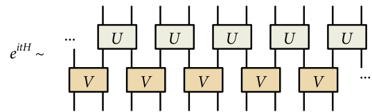
FIG. 2 (color online). The approximate quantum cellular automata decomposition for e^{itH} for time t . Each of the unitary operators U and V acts on at most c_0|t| spins, where c_0 is a constant.
