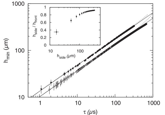
FIG. 2. Scaling of h_{\min} versus \tau for bubbles released quasistatically in water from circular nozzles of R_N = 1.5 \text{ mm} (open circles) and 4.1 \text{ mm} (solid circles). The Reynolds numbers in water at the beginning of detachment are approximately 0.6 and 4, respectively. The solid lines show power-law fits with exponent \alpha_h = 0.56 , and the dashed lines show fits with logarithmic corrections [14,24]. Data are taken from multiple pinch-offs, and only data for \tau \leq 230 \mu\text{s} are used for fitting. Inset: For the tilted-nozzle image sequences shown in Fig. 3(a), the radial size of the neck scales differently in the front ( h_{\text{front}} ) and side ( h_{\text{side}} ) directions.
