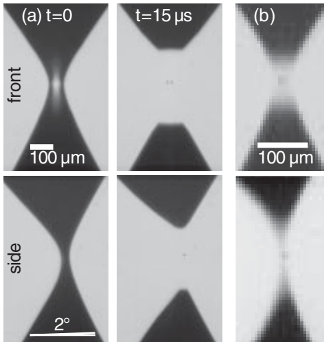
FIG. 3. Front and side views of pinch-off from an R_N = 4.1 mm nozzle tilted by 2^\circ . The nozzle's tilt is indicated in the bottom-left frame; in the front images, it is tilted away from the camera. Front and side images are from separate sequences but were selected to match length scales closely. (a) The neck is broadened before the breakup, resembling a crimped and bent double cone. A pair of satellite bubbles \sim 15 \mu\text{m} in diameter is produced. Afterward, the tip of each interface is bifurcated. (b) In these 2 \mu\text{s} exposures, the final form of the neck is captured along with the initial positions of the satellite bubbles. The neck reaches zero thickness while it is still \sim 20 \mu\text{m} wide, resulting in what appears to be a rupture instead of a smooth, symmetric pinch-off.
