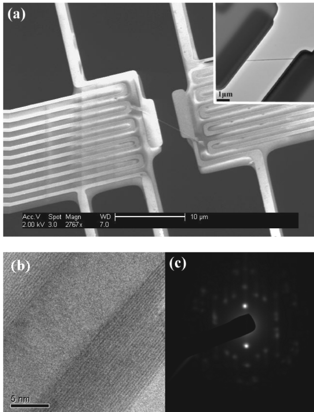
FIG. 1. (a) A scanning electron microscope image of the microfabricated test fixture with a boron nitride nanotube on it (scale bar = 10 μm). The inset shows the corresponding transmission electron microscope image of the same device (scale bar = 1 μm). (b) A high-resolution transmission electron microscope image of the boron nitride nanotube (scale bar = 5 nm). (c) The corresponding electron diffraction pattern of the boron nitride nanotube.
