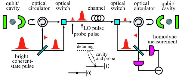
FIG. 1 (color online). Schematic for the generation of spin entanglement between two qubits at neighboring stations via homodyne detection discriminating between conditionally phase-rotated coherent probe beams; the LO pulse is a sufficiently strong local oscillator used for the homodyne detection.
