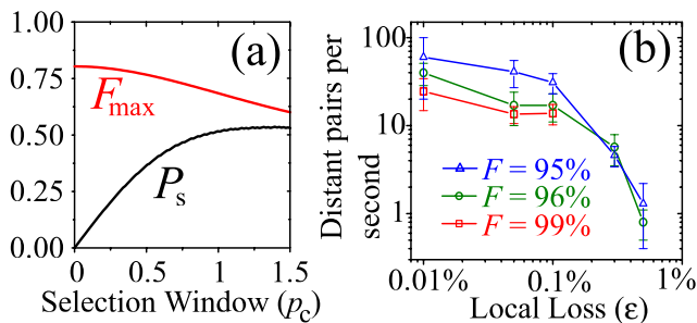
FIG. 2 (color online). (a) The maximum fidelity F_{\text{max}} and success probability P_s as a function of the postselection window p_c for \eta^2 = 2/3 . (b) Achievable qubit rates for different target fidelities vs local optical losses \epsilon . Each point corresponds to a single Monte Carlo simulation of the nested purification protocol over 9 complete qubit teleportations; each point is the average difference in time between teleported qubit arrival times, and the error bar is the standard deviation.
