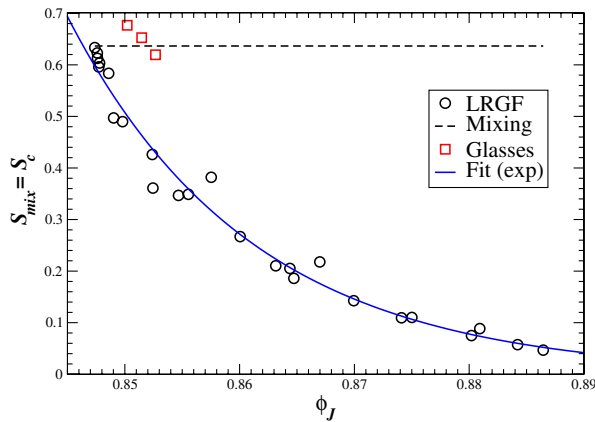
FIG. 5 (color online). The measured degeneracy of packings of N = 4096 disks obtained by using different parameters of a random Gaussian field with Matern correlations [18], as a function of the jamming density. For comparison, we have shown s_c(\phi = 0.825) for the three compressions shown in Fig. 3.
