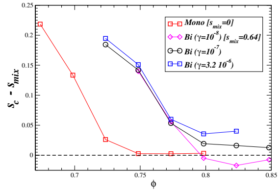
FIG. 3 (color online). Estimated s_c(\phi) - s_{\text{mix}} for monodisperse and bidisperse systems of N = 4096 disks, as obtained from (sufficiently slow) compressions with a range of \gamma 's.
