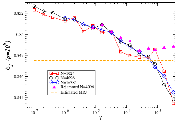
FIG. 2 (color online). Final jamming density \phi_J for different compression rates \gamma , with and without additional relaxation to ensure a truly jammed packing has been reached.
