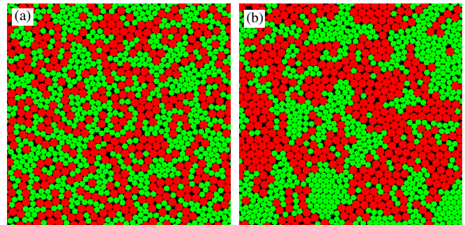
FIG. 4 (color online). The microstructures of two packings: (a) without ( \phi_J \approx 0.846 ) and (b) with moderate clustering ( \phi_J \approx 0.850 ).
