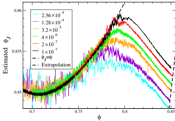
FIG. 1 (color online). The equation of state \bar{\phi}_J(\phi) for N = 4096 disks as observed by compressing a liquid with different expansion rates \gamma (see legend).
