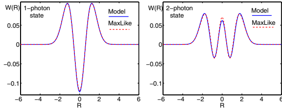
FIG. 4 (color online). Experimental Wigner functions corrected for losses in the homodyne detection, reconstructed by a standard maximal-likelihood (MaxLike) method, compared to those obtained using the model described in the text.
