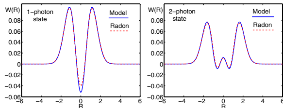
FIG. 3 (color online). Wigner functions of the measured uncorrected states, reconstructed by a standard Radon transform, compared to those obtained using the model described in the text.
