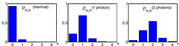
FIG. 5 (color online). Main density matrix coefficients of the states conditioned on 0, 1, and 2 photons (corrected for detection losses).
