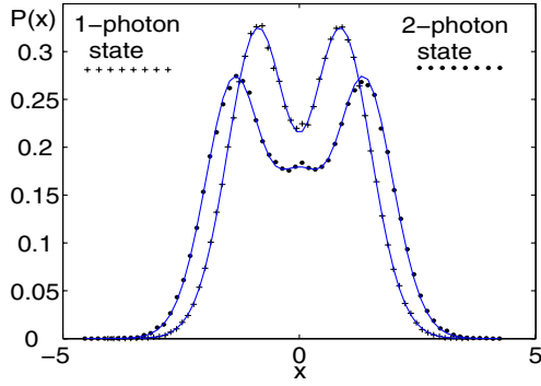
FIG. 2 (color online). Experimental quadrature measurements and quadratures reconstructed using our model (see text).
