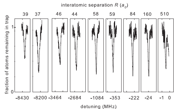
FIG. 3. The spectra of the long-range \text{Sr}_2 molecule near the ^1S_0 - ^3P_1 dissociation limit. The horizontal scale is marked on the rightmost panel and is the same for each of the nine blocks; different PA laser intensities were used for each spectrum due to largely varying line strengths. The top labels indicate the interatomic separations that correspond to the classical outer turning points of each resonance.
