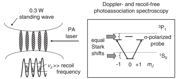
FIG. 2. Experimental configuration. The 2 \mu\text{K} atoms are confined in a 1D optical lattice in the Lamb-Dicke regime that allows Doppler- and recoil-free photoassociation spectroscopy. The lattice laser intensity is large enough to confine most atoms in the ground motional state. The 689 nm weak PA laser copropagates with the lattice. The 914 nm lattice wavelength ensures that ^1S_0 and the m_J = \pm 1 sublevels of ^3P_1 are Stark shifted by equal amounts.
