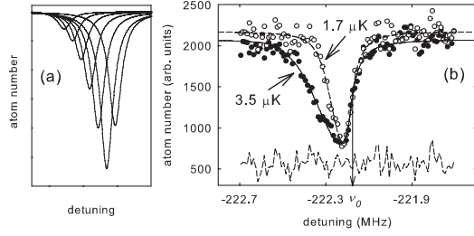
FIG. 4. (a) A line is schematically shown as a sum of Lorentzians with positions and amplitudes given by a continuous thermal distribution. (b) The measured line shapes of the -222 MHz transition at 1.7 \mu\text{K} (open circles) and 3.5 \mu\text{K} (solid circles), clearly showing the effect of temperature on the red side of the line. The bottom trace shows the residuals of the 1.7 \mu\text{K} curve fit.
