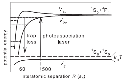
FIG. 1. Schematic diagram of the long-range Sr 2 molecular potentials (not to scale). The ground and excited molecular states coincide with two ground state atoms, and with one ground and one excited state atom, respectively, at large internuclear separations. The ground state has gerade symmetry and its energy is given by the potential V_g , while the excited state ungerade potentials that support dipole transitions to the ground state are V_{0u} and V_{1u} , the latter with a small repulsive barrier. All vibrational states of 0 u and 1 u (dashed and dotted lines, respectively) are separated by more than the natural line width, permitting high resolution PA spectroscopy very close to the dissociation limit when the atoms are sufficiently cold.
