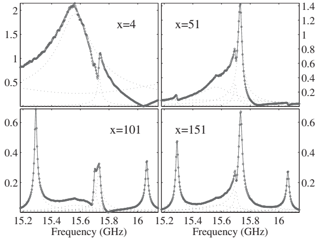
FIG. 3. Comparison of the measured field magnitude (dots) to Eq. (1) (full line) at four different locations. The Lorentzian lines and the polynomial in Eq. (1) are represented by dotted lines.
