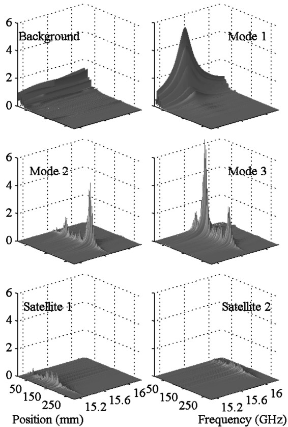
FIG. 5. Field magnitude for five quasimodes and slowly varying polynomial term in Eq. (1).
