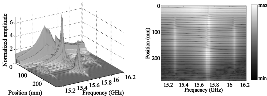
FIG. 2. (a) Spectra of the field amplitude at each point along a random sample with spectrally overlapping peaks normalized to the amplitude of the incident field. (b) The top view of (a) in logarithmic presentation.
