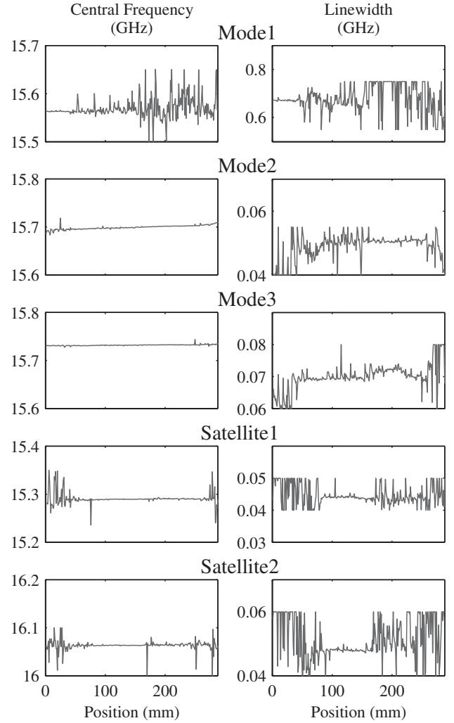
FIG. 4. Spatial dependence of central frequency and linewidth for the five modes shown in Fig. 5. At positions at which the mode amplitude is greater than the noise, the central frequency and linewidth are sharply defined.
