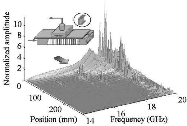
FIG. 1. Spectra of the field amplitude at each point along a typical random sample normalized to the amplitude of the incident field. The arrow points to the input direction. Inset: Description of the experimental set up and schematic of the ceramic structure element.
