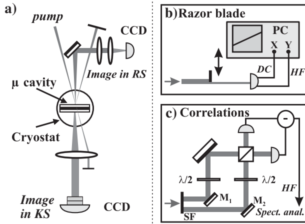
FIG. 1. (a) Experimental setup. CCD camera for images in RS (KS) of the emitted light in reflection (transmission). (b) “Razor blade” setup. HF (DC), high (low) frequency part of the signal. PC means computer. (c) Intensity correlations setup. Each of the mirrors M_1 and M_2 reflects the emission from one of the regions selected by the spatial filter (SF) in KS [see also Fig. 2(b)].
