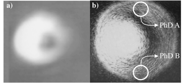
FIG. 2. Image of the nonlinear emission (a) in RS and (b) in \mathbf{k} space in the degenerate geometry [16]. Cavity-exciton detuning 0.3 meV and laser intensity 2.2 mW. In (a) the dark region in the laser spot corresponds to the polariton resonance. In (b) the polariton emission is seen around the (brighter) reflected laser in \mathbf{k} space, showing a larger angular divergence. The principle of the intensity correlation measurement is schematically indicated.
