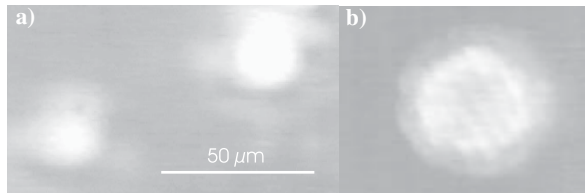
FIG. 4. Image of the light emitted in a cone of 2^\circ around the normal direction (a) in RS in reflection and (b) in \mathbf{k} space in transmission. Cavity-exciton detuning: 1.3 meV. Laser intensity: 2.8 mW (around 1.5 times the threshold intensity).
