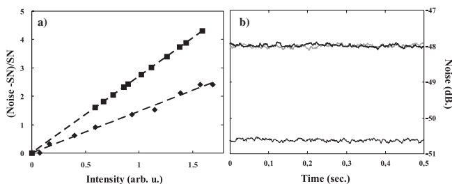
FIG. 3. (a) Squares (diamonds): variations of the noise—HF signal—of the nonlinear emission around \mathbf{k} = \mathbf{0} as a function of the detected intensity—DC signal—in the degenerate (nondegenerate) geometry. The shot noise (SN) is subtracted from the total noise, and the result is normalized to the SN. Cavity-exciton detuning: respectively, 0.3 and 1.2 meV. In the degenerate case, points at very low intensity are missing because the noise was too small compared to dark noise. (b) Noise power as observed on the screen of the spectrum analyzer. Black line: noise of the intensity difference, perfectly superimposed with the shot noise level (gray line). Dark noise (lower gray line) is 2.6 dB below the SN level.
