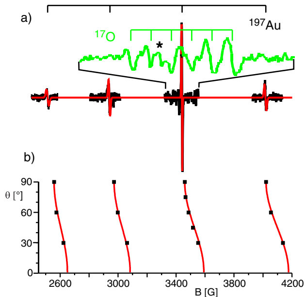
FIG. 1 (color online). (a) Experimental and simulated EPR spectrum of Au atoms adsorbed on MgO(001)/Mo(001) ( \theta = 90^\circ ), green trace: spectrum for an 17 O enriched MgO film (signal marked by a * belongs to the background). (b) Angular dependence of EPR resonance positions with respect to the polar angle \theta between static magnetic field and surface normal.
