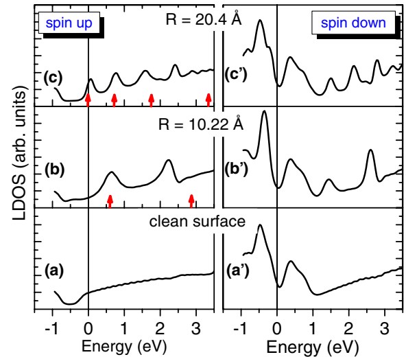
FIG. 2 (color online). LDOS for (b),(c) the majority and (b'),(c') the minority surface-state electrons at the center of hexagonal Cu corrals; (a),(a') show LDOS of the surface-state electrons on an open 2 ML Co/Cu(111). Predictions of the analytical model for the peak positions in LDOS(spin-up) are marked by arrows.
