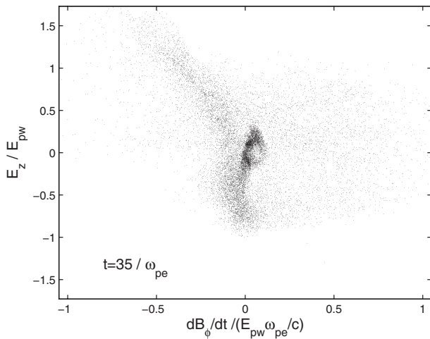
FIG. 3. Correlation of longitudinal electric field with time variation of azimuthal magnetic field at the same spatial location for a 10\lambda_p long, 6\lambda_p wide jet. For clarity, only a random subset of field points outside a radius of 2.5\lambda_p are shown.
