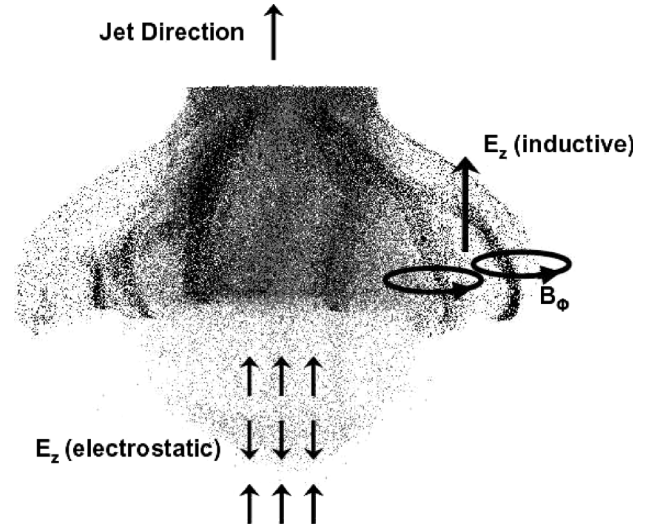
FIG. 2. Side view of a 10\lambda_p long, 6\lambda_p wide jet at simulation time t = 35\omega_{pe}^{-1} , showing positron filaments (black dots) expelled from the jet leaving behind the electrons (gray dots). It also illustrates the mechanisms for generating inductive as well as electrostatic longitudinal electric fields.
