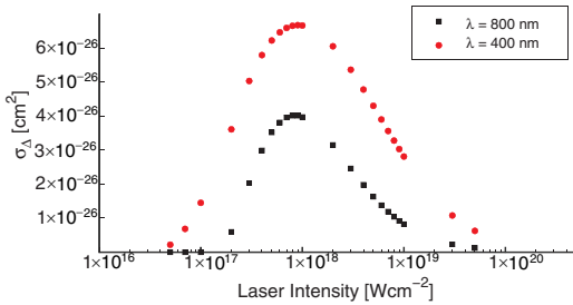
FIG. 3 (color online). The average cross section, \sigma_{\Delta} , for inverse Compton scattering of incident light with wavelength 800 nm and 400 nm into the wavelength interval 216–316 nm, as a function of increasing intensity of the incident light.
