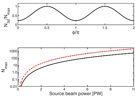
FIG. 2 (color online). The upper panel shows the number of scattered photons N_{3d} per shot, normalized by the number of photons N_{\max} per shot for an optimal choice of polarization, as a function of polarization angle \phi of the wave with direction \hat{\mathbf{k}}_3 . The lower panel shows N_{\max} predicted by (8) when increasing the laser power while keeping the beam width constant at b = 1.6 \mu m, for a system where two source beams are used and one of the beams is split into two (solid line) and when three source beams are used, hence no beam splitting is required (dashed line).
