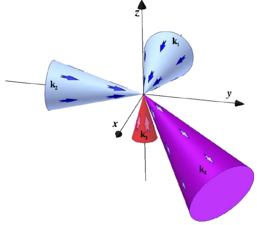
FIG. 1 (color online). Configuration of the incoming laser beams and the direction of the scattered wave for the suggested three-dimensional configuration of wave vectors, which satisfies the matching conditions (5).
