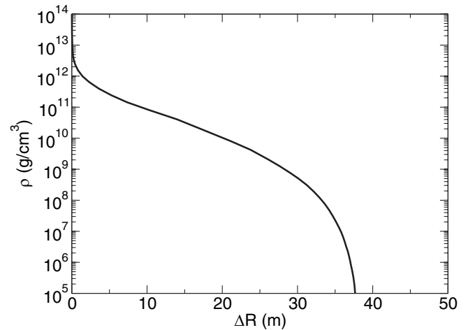
FIG. 2. Density profile of the crust for a strange star with mass M = 14M_\odot and radius R = 10 km.
