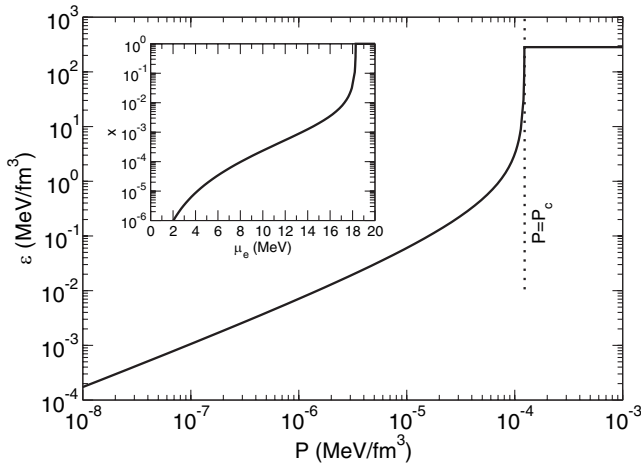
FIG. 1. The equation of state of the mixed phase. Inset shows the variation of the volume fraction of the quark phase as \mu_e changes across the mixed phase.
