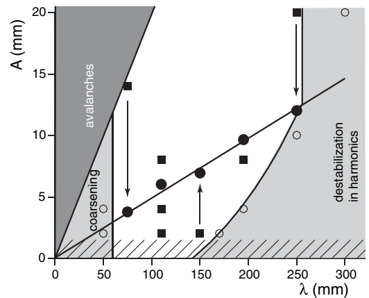
FIG. 4. Stability diagram of ripples of initial wavelength \lambda and amplitude A for u^* = 1.3u_{th} . Outside the locking zone (○), the pattern destabilizes by generation of harmonics (right) or subharmonics (left). Starting in the central region (■), \lambda stays constant and A readapts to reach a stable steady solution (●). Very large amplitudes cannot be imposed as avalanche processes take place. Hatched region is beyond experimental access.
