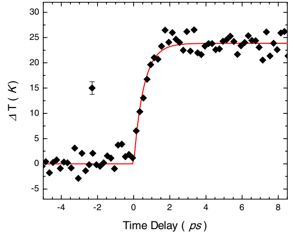
FIG. 3 (color online). Temporal evolution of lattice temperature as a function of delay time. The solid line is a fit to the data using an exponential function with a time constant t_{e-ph} = 550 \pm 80 fs.
