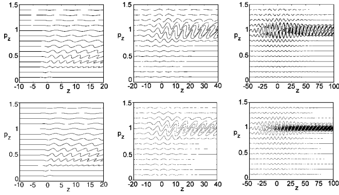
FIG. 1. Numerically (top) and analytically (bottom) obtained Poincaré surfaces of section for interaction with a SW having A_1 = 0.005 , \sigma_1 = 1, 10, 30 (left to right), \omega_1 = 1 , v_{p_1} = 1 , v_{g_1} = 0 .
