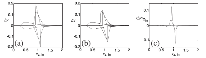
FIG. 2. Numerically (a) and analytically (b) obtained extrema of particle velocity variation \Delta v for interaction with a SW having A_1 = 0.005 , \sigma_1 = 1, 10, 30 , \omega_1 = 1 , v_{p_1} = 1 , v_{g_1} = 0 . Larger values for \sigma_1 result in stronger localization of the resonant velocity area. (c) Position-averaged particle velocity variation.
