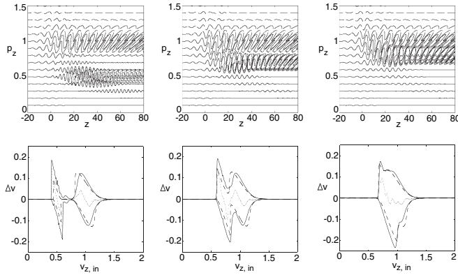
FIG. 3. Interaction with two SWs. (Top) Numerically obtained Poincaré surface of section. (Bottom) Numerically (solid) and analytically (dashed) obtained extrema of velocity variation. The averaged velocity variation is also shown (dotted line). The parameters of the SWs are A_{1,2} = 0.005 , \sigma_{1,2} = 10 , \omega_{1,2} = 1 , v_{g_1} = 0 , v_{g_2} = 0.1 , v_{p_1} = 1 , v_{p_2} = 0.5, 0.7, 0.8 (left to right).
