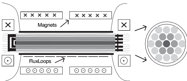
FIG. 1. A schematic of the line-tied pinch experiment. The solenoidal magnets produce a nearly uniform magnetic field between the two ends. The anode plate is on the left and drawn to highlight its electrical connectivity. The hexagonally packed cathode array of plasma guns (shown on the right) breaks into three independently controllable regions of plasma represented by shadings in gray. The flux loops are shown in relation to the machine.
