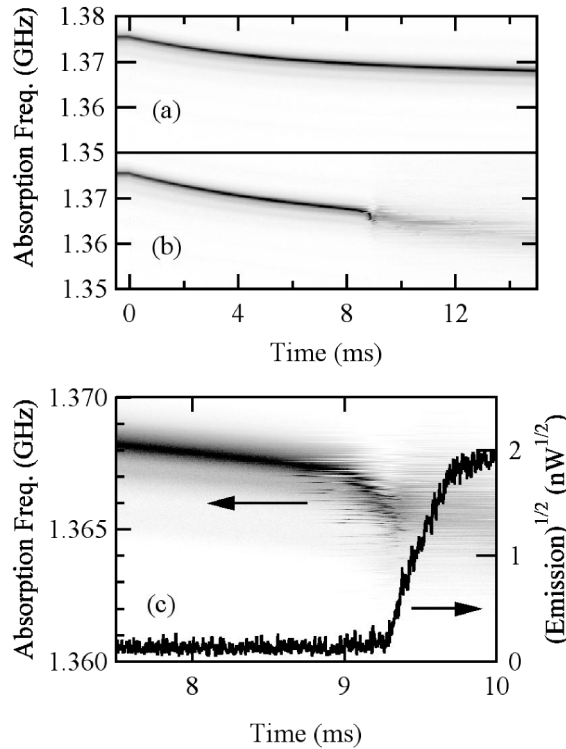
FIG. 1. AFMR absorption vs time in the presence of a low frequency driver. f_2 = 1.330 GHz. Darker density represents stronger absorption. (a) Driver power = 1.1 W and (b) Driver power = 1.4 W. At about 9 ms a transition occurs to a broadened resonance. (c) Enhanced view of the broadening transition at 9 ms in (b). The four-wave mixing (emission) 1/2 is superimposed. The nonlinear emission step occurs in tandem with the broadening of the AFMR.
