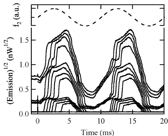
FIG. 3. (\text{Emission})^{1/2} vs time during f_2 power modulation. Solid lines plot the ILM emission as f_2 is modulated at 100 Hz and scanned from 112 to 200 mW in 4.7% increments from bottom to top. The 25% sine wave amplitude modulation begins at t = 0 ms. The dashed curve illustrates the time pattern of f_2 . The emission has a phase shift of \sim -\pi/5 relative to the driver.
