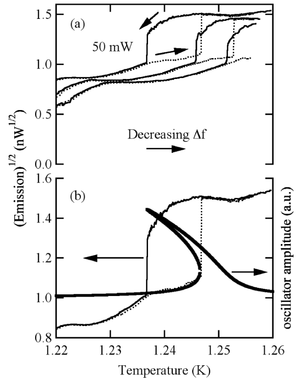
FIG. 2. Step hysteresis in (emission) 1/2 vs temperature. (The abscissa also identifies the linear temperature dependence of the AFMR frequency in the presence of the f_2 driver.) (a) f_2 = 1.350 GHz with three powers: 50 mW, 47.4 mW, and 45.7 mW. Dotted lines: increasing temperatures; solid lines: decreasing temperatures. The hysteresis due to capture and loss of a single ILM is evident. (b) Comparison of the 50 mW data with a model. Thick line: hysteresis characteristic of the amplitude response for a driven nonlinear oscillator.
