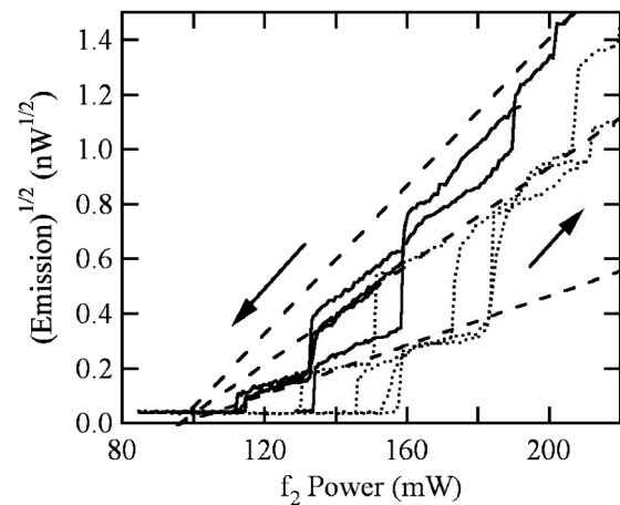
FIG. 4. (\text{Emission})^{1/2} at constant times as a function of f_2 power. The traces extracted from Fig. 3 are separated by 1.25 ms. Dotted data lines: 10–15 ms (ILM creation); solid data lines: 15–20 ms (ILM loss). The f_2 power on the abscissa is calculated separately for each slice, and includes a phase shift of -\pi/5 to that of the applied field. The dashed lines are guides to the eye that follow the proportionality given in Eq. (1).
