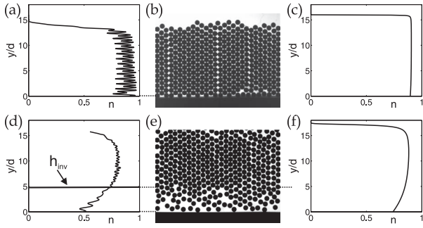
FIG. 2. (a) Density profile, averaged over 300 consecutive snapshots, as a function of height for F = 16 layers at shaking strength \Gamma = 7.7 ( a = 0.3 mm, f = 80 Hz). The origin y/d = 0 is set at the maximal positive displacement of the vibrating bottom. (b) A typical snapshot of this experiment recorded by a high-speed camera (1000 fps) and (c) the theoretical profile from the model in Eqs. (4)–(6) with S = 4.0 . (d) Density profile for F = 16 layers at \Gamma = 51.5 ( a = 2.0 mm, f = 80 Hz), showing the Leidenfrost state. The inversion height h_{\text{inv}} marks the border between the gaseous and the solid phase; it is determined via the method illustrated in Fig. 3. (e) The corresponding experimental snapshot and (f) the theoretical profile for S = 80 .
