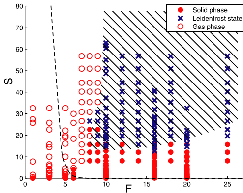
FIG. 5 (color online). Phase diagram of F (number of layers) vs S (shaking strength), with the Leidenfrost state showing up between the regions of solid and gaslike behavior. The symbols represent experimental data: solid phase ( \bullet ), gas phase ( \circ ), and Leidenfrost state ( \times ). The shaded area is the Leidenfrost regime according to our hydrodynamic theory. The dashed curve marks the onset of density inversion at the bottom, dn/dy|_{y=0} = 0 , an essential precursor to the Leidenfrost effect.
