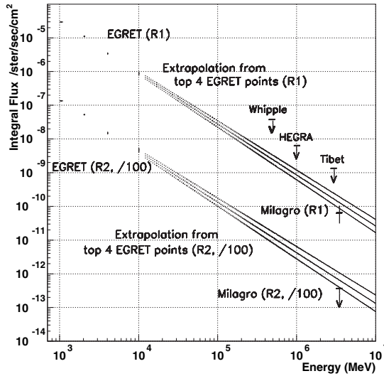
FIG. 4. Integral flux results of Milagro and EGRET detectors, with 99% C.L. upper limits from Whipple [ l \in (38.5^\circ, 41.5^\circ) , |b| < 2^\circ ] [8], HEGRA [ l \in (38^\circ, 43^\circ) , |b| < 5^\circ ] [9], Tibet [ l \in (20^\circ, 55^\circ) , |b| < 5^\circ ] [10]. The display for region R2 is shifted by 10^{-2} .
