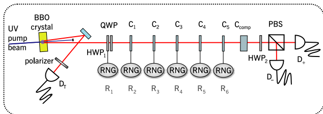
FIG. 2 (color online). Setup for single qubit secret sharing. Pairs of orthogonally polarized photons are generated via a type II SPDC process in a BBO crystal. The detection of one photon from the pair by D_T heralds the existence of the other one used in the protocol. The initial polarization state is prepared by placing a polarizer in front of the trigger detector. Each of the recipients ( R_1 \dots R_6 ) introduces one out of four phase shifts, according to the output of a pseudorandom number generator (RNG), using half- and quarter-wave plates ( \text{HWP}_1 , QWP) or \text{YVO}_4 crystals ( C_1 \dots C_5 ), respectively. The last party analyzes additionally the final polarization state of the photon by detecting it behind a half-wave plate ( \text{HWP}_2 ) and a polarizing beam splitter (PBS).
