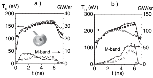
FIG. 2. Radiation temperature history as measured by Dante through LEH (thick solid line) and as simulated by LASNEX (full squares). Circles are predicted internal radiation temperatures. Measured (thin solid line) and calculated (triangles) M -band ( >2 keV) flux are plotted on the right scale. (a) scale-3/2 and (b) scale-1 hohlraums driven by 2.7 TW in 6 ns flattop laser pulse. Dante view of typical hohlraum target with initial laser spots on the wall shown as dark circle shown as inset on (a).
