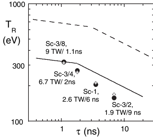
FIG. 3. Dante measured temperatures T_{LEH} at the rollover time \tau and the corresponding analytical limits (crosses) calculated with Eq. (6) using experimental values of LEH radius r and laser power. Continuous and dashed black lines are Eq. (6) analytic model limits for a constant LEH radius r = 0.3 mm for 9 TW, 16 kJ 1 quad NIF hohlraums and for 600 TW, 1.8 MJ NIF hohlraum.
