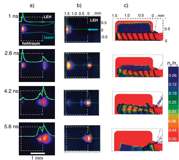
FIG. 1 (color). Side-on hard x-ray gated images and the corresponding axial intensity profiles (a) measured and (b) calculated in scale-1 hohlraum heated by 2.7 TW, 6 ns laser pulse. (c) Cross-section of electron density profiles and laser ray propagation calculated with 2D LASNEX code.
