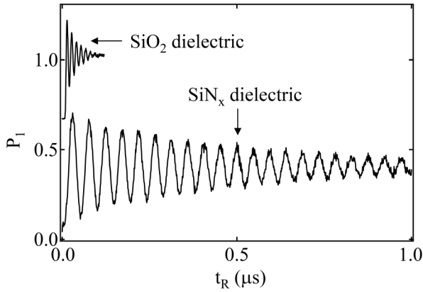
FIG. 3. Rabi Oscillations for a phase qubit using CVD SiO 2 (top trace, offset) and SiN (bottom trace) as a dielectric for the crossover wiring. Microwaves at the qubit frequency are pulsed for a time t_R , and subsequent measurement of the qubit state shows an oscillation of the probability of the excited state. The decay of the Rabi oscillations is consistent with the measured relaxation time of T_1 = 0.5 \mu\text{s} , which is about 20 times better than previous experiments with a SiO 2 dielectric. From Ramsey fringes, we determined a dephasing time of T_2 = 150 \text{ ns} (data not shown).
