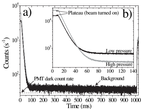
FIG. 2. Typical time-normalized decay curves for two series of measurements taken at different injection gas pressures, as reflected in the heights of the plateaus: (a) is for 1 s beam off time ( 111.1 \mu\text{s}/\text{channel} ), and (b) is for 200 ms beam off time ( 50 \mu\text{s}/\text{channel} ).
