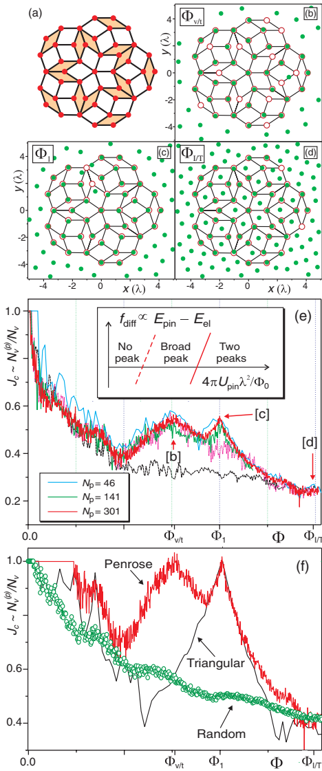
FIG. 2 (color online). (a) An example of a fivefold Penrose lattice, consisting of thick and thin rhombuses. (b)–(d) The location of vortices (green dots) and the Penrose-lattice APS (red open circles connected by black lines) for (b) \Phi = \Phi_{\text{vacancy/thin}} \equiv \Phi_{v/t} = 0.757\Phi_1 , vortices occupy all the pinning sites except those in one of the two vertices of each thin rhombus; (c) \Phi = \Phi_1 , N_v coincides with N_p ; (d) \Phi = \Phi_{\text{interstitial/thick}} \equiv \Phi_{1/T} = 1.482\Phi_1 , vortices occupy both the pinning sites and the interstitial positions inside each thick rhombus. Here f_p/f_0 = 2.0 , r_p = 0.1\lambda . (e) The J_c(\Phi \sim N_v) for Penrose-lattice arrays with N_p = 46, 141, 301 . The data points [b], [c], [d] refer to snapshots in 2(b)–2(d), respectively. The peak [c] at \Phi_1 is suppressed for weaker pinning (magenta dotted J_c curve). Eventually, all the main peaks disappear for sufficiently weak pins (black dashed curve). The inset shows the dimensionless difference, f_{\text{diff}} , of the pinning and the elastic energies versus the pinning-to-interaction energy ratio, for the broad J_c peak at \Phi_{v/t} (red dashed line) and for \Phi_1 (red solid line). Only f_{\text{diff}} > 0 gives stable peaks in J_c . (f) The J_c(\Phi) for a 301 sites Penrose lattice (red solid line), (recalculated for flux only on the Penrose area, A_p ), triangular (black solid line), and random (green open circles and solid line) pinning arrays.
