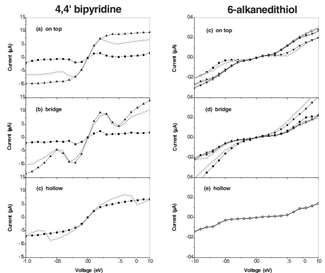
FIG. 3. Current-voltage characteristics for Au-4,4'-bipyridine-Au wires (left panel) and Au-alkanedithiol-Au wires (right panel) on different binding sites. The molecule is set perpendicular to the electrode surface, and rotated for multiples of \frac{\pi}{4} along its axis. Different symbols correspond to rotations along the molecular axis for every \frac{\pi}{4} (equivalent configurations are not included).
