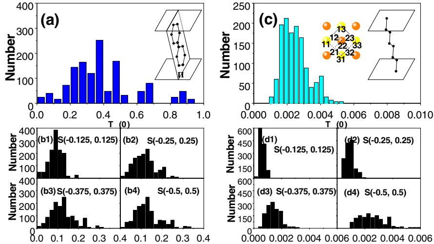
FIG. 1 (color online). Statistical analysis of transport properties for molecular wires with different binding sites and orientations. The distance between the two Au lead surfaces is fixed at 11.38 \text{ \AA} for bipyridine wires and 12.38 \text{ \AA} for alkanedithiol wires. Each N atom in bipyridine and each S atom in alkanedithiol can bind to one of the nine sites marked in the middle inset of (c). (a) Histogram of transmission coefficient at Fermi energy, T(0) , for the ensemble of bipyridine wires. Inset: schematic showing an approximate geometry of the bipyridine wires. (b)1)–(b)4) histograms of the quantity S(E_1, E_2) in different energy ranges for the bipyridine wires. (c) Histogram of T(0) for the ensemble of alkanedithiol wires. Middle inset: the numbers indicate binding sites in the ensemble. Right inset: schematic showing an approximate geometry of the alkanedithiol wires. (d)1)–(d)4) Histograms of S(E_1, E_2) for the ensemble of alkanedithiol wire.
