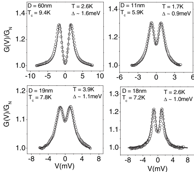
FIG. 3. Point contact Andreev reflection spectra for nanostructured Nb samples with T_c = 9.4, 7.8, 7.2, and 5.9 K. The open circles show the conductance data (normalized to the conductance in the normal state) while the solid line is the fit to the Blonder-Tinkham-Klapwijk theory.
