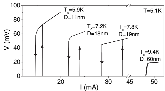
FIG. 2. I - V characteristics (with increasing and decreasing current) of the nanostructured Nb samples with T_c = 9.4 , 7.8, 7.2, and 5.9 K measured at 5.1 K. The sample with an average size ( D ) of 60 nm shows bulklike behavior.
