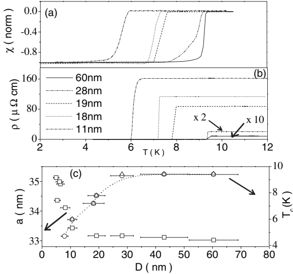
FIG. 1. Temperature dependence of (a) magnetic susceptibility ( M/H ), and (b) resistivity in nanostructured thin films of Nb with different average particle size. (c) Size dependence of the superconducting transition temperature ( T_c ) obtained from magnetization (open circles) and resistivity (open triangles) measurements (scale on right). (c) Also shows the size dependence of the lattice parameter (open squares) in nano-Nb (scale on left). The width of the measured size distribution is indicated by the error bars.
