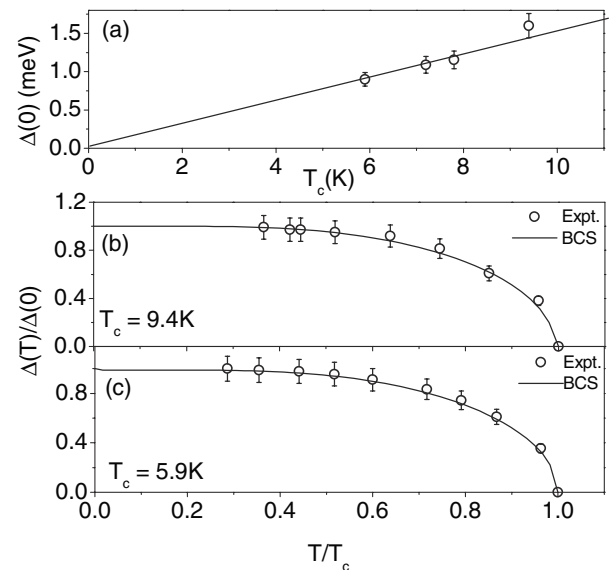
FIG. 4. (a) Variation of superconducting gap \Delta(0) with the T_c , and (b) temperature dependence of \Delta(T) with the reduced temperature for two typical samples of nano-Nb, with T_c = 5.9 K, and T_c = 9.4 K.
