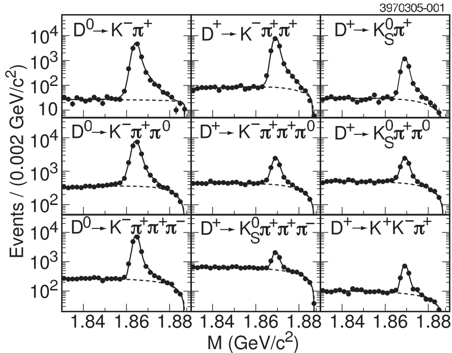
FIG. 1. Semilogarithmic plot of ST yields and fits, with D and \bar{D} combined for each mode. Data are shown as points with error bars. The solid lines show the total fits and the dashed lines the background shapes. The high mass tails on the signal are due to initial state radiation.
