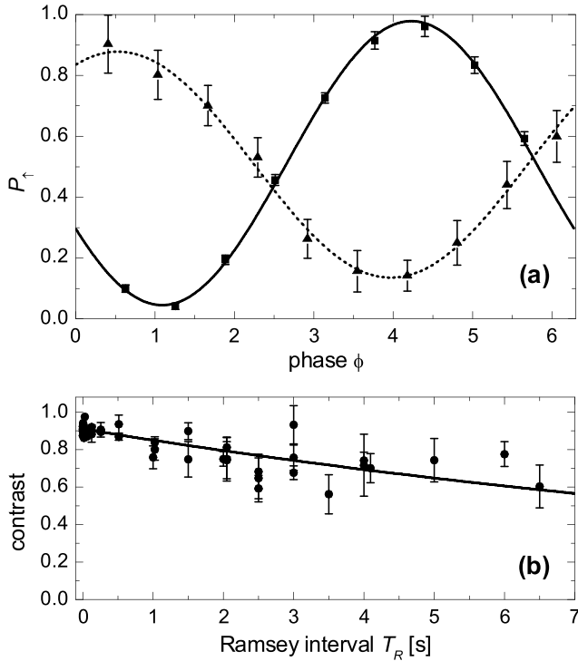
FIG. 3. (a) Ramsey data at T_R = 4 ms (squares) and 4 s (triangles). The y axis represents the probability of measuring the state |\uparrow\rangle . The contrast b for the 4 ms data is 0.933 \pm 0.014 and for the 4 s data is 0.742 \pm 0.043 . The \phi_D \approx 1 rad phase shift in the 4 ms data is due to detuning the local oscillator by the differential Stark shift ( \sim 4.2 kHz) such that the Ramsey \pi/2 pulses are resonant. (b) Contrast vs Ramsey interval T_R . Each datum represents the fitted contrast b for a phase scan with Ramsey interval T_R . The solid curve is a weighted least-squares fit to the data with reduced \chi^2 \approx 1.16 .
