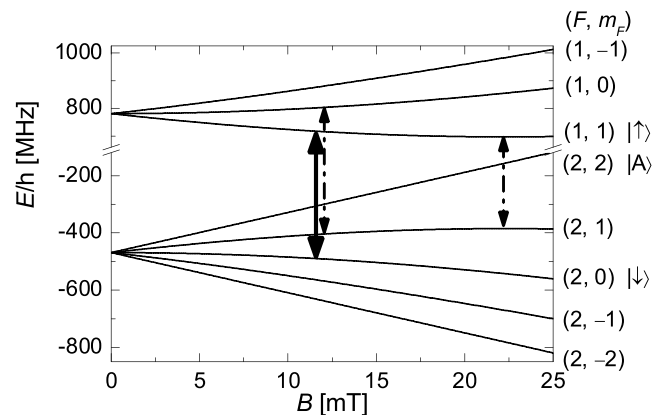
FIG. 1. Hyperfine level structure of the 2s\ 2S_{1/2} state of {}^9\text{Be}^+ . The solid arrow indicates the magnetic-field-independent transition studied here (0.01194 T); the dashed arrows indicate other useful field-independent transitions at 0.01196 T and 0.02231 T.
