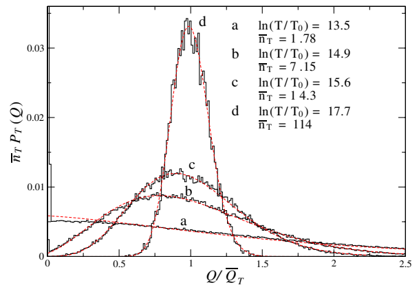
FIG. 2 (color online). Evolution of the full counting statistics P_T(Q) for four different time intervals T with \lambda = 4.0 and eV = 3\hbar\omega_v . The MC data (solid lines) are in excellent agreement with the analytical full counting statistics, Eq. (6) (dashed lines), with \bar{N}^{(0)} = 91.2 , \bar{n}_T = 2.4 \cdot 10^{-6} T/T_0 (no fit), and T_0 = (2\pi\rho t_0^2/\hbar)^{-1} .
