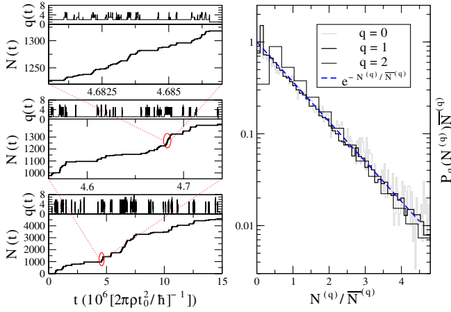
FIG. 1 (color online). Hierarchical character of transport. Left: Three generations of self-similar MC plots for \lambda = 4 and eV = 3\hbar\omega_v , showing the net-transferred charge N and phonon state q as functions of time. ( \omega_v : phonon frequency; \rho : density of states of the leads; t_0 : molecule-lead coupling). Right: Comparison of the fixed-point distribution for the transferred charge per generation- q avalanche to numerical simulations for q = 0, 1, 2 (mean values \bar{N}^{(0)} = 91.2 , \bar{N}^{(1)} = 11.1 , and \bar{N}^{(2)} = 2.9 ).
