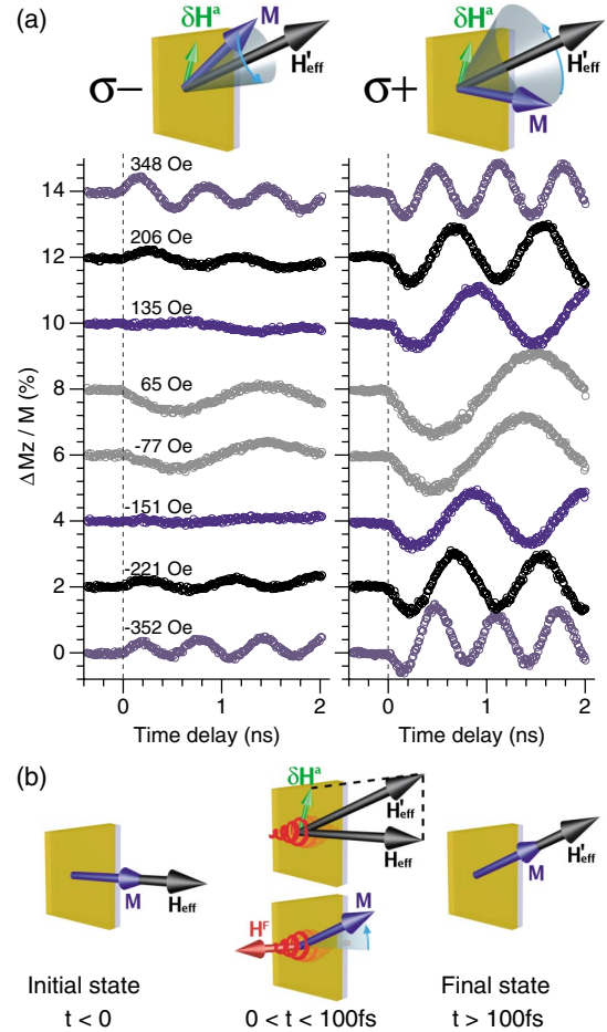
FIG. 3 (color). All-optical switching of the magnetization within 100 fs. (a) Precession of the magnetization triggered by left- and right-hand circularly polarized laser pulses at different values of the in-plane applied magnetic field. For the \sigma^- helicity, at an applied field of \sim \pm 150 Oe, no precession is observed due to a perfect balance of the two photomagnetic effects. (b) Graphical illustration of the switching process: Initially at t < 0 the magnetization is along \mathbf{H}_{\text{eff}} . During the presence of the laser pulse 0 < t < 100 fs photoinduced modification of the anisotropy fields leads to a new metastable equilibrium along \mathbf{H}'_{\text{eff}} . Simultaneously, the strong optically generated field \mathbf{H}^F causes the magnetization to precess into the new state. After t > 100 fs the optical pulse is gone and the 0.6^\circ switching of \mathbf{M} is complete.
