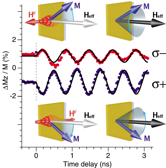
FIG. 2 (color). Precession of the magnetization following excitation with circularly polarized light. The two helicities \sigma^+ and \sigma^- give rise to precession with opposite phase and different amplitude. During the presence of the laser pulse 0 < t < 100 fs the magnetization precesses in the dominating axial field \mathbf{H}^F . Subsequent precession takes place in the effective magnetic field composed of anisotropy fields and the externally applied field.
