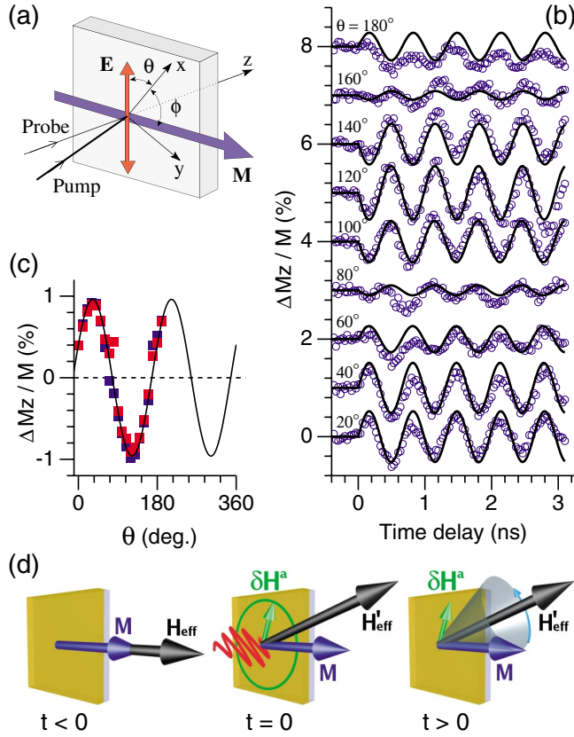
FIG. 1 (color). Coherent precession of the magnetization triggered by a change in anisotropy field \delta\mathbf{H}^a induced by linearly polarized laser pulses. (a) Experimental geometry: A garnet film with in-plane magnetization \mathbf{M} at an angle \phi with respect to the crystallographic x axis. \theta denotes the angle between the plane of polarization of the linearly polarized pump pulses and the x axis. (b) Time dependence of the precession for different planes of polarization \theta , with an applied field of |\mathbf{H}_{\text{ext}}| = 350 Oe in the plane of the sample. Circles represent measurements and solid lines represent simulations based on the Landau-Lifshitz equation. (c) Precessional amplitude as a function of the plane of polarization. Red and blue symbols represent amplitudes extracted from measurements at \pm\mathbf{H}_{\text{ext}} . The solid line is a best fit. (d) An illustration of the excitation process and the subsequent precessional dynamics.
