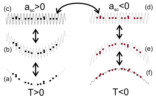
FIG. 4 (color online). Method for reversibly transforming a positive-temperature gas (a) into a negative-temperature gas (f). Each step is reversible; see text. (a) trapped gas at positive T , (b) a strong optical lattice, (c) a strong optical lattice without trap, (d) a strong optical lattice with changed a_{\text{sc}} , (e) a strong optical lattice with negative trap, (f) an optical lattice at q = 0.936 with a negative-temperature gas.
