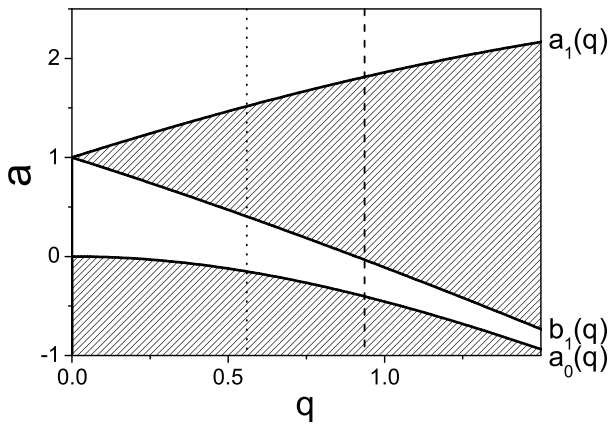
FIG. 1. Band structure of the one-dimensional Mathieu equation. White area: Bands, gray area: gaps. Dotted line: q = 0.559 , dashed line: q = 0.936 ; see text.
