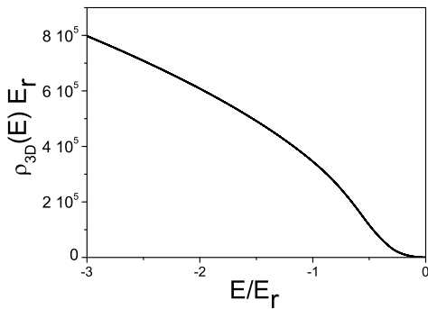
FIG. 3. Density of states \rho(E) in a three-dimensional lattice with \tilde{\alpha} = -10^{-3} . The energy E is taken with respect to the top of the first (valence) band.
