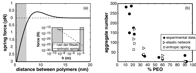
FIG. 3. (a) Expected value for the network force function and an order-of-magnitude comparison with van der Waals forces (inset). The gray shaded region in the spring force function indicates forbidden separation distances due to the incompressibility of the PEO pancake ( R_{PEO} is approximately 7 nm for this polymer). Grey regions in the inset indicate film thicknesses that are outside of the normal range sampled by the polymer film as the solvent evaporates during the course of the experiment. (b) Comparison of model predictions for the aggregate number with experimental data. Triangles and squares indicate two different network force functions: triangles correspond to the function given in the text, and squares correspond to a logarithmic entropic spring function [20]. The two experimental parameters that play a role in determining the aggregate number are the percentage of PEO and N ; each data point corresponds to a particular (% PEO, N ) pair as summarized in Table I.
