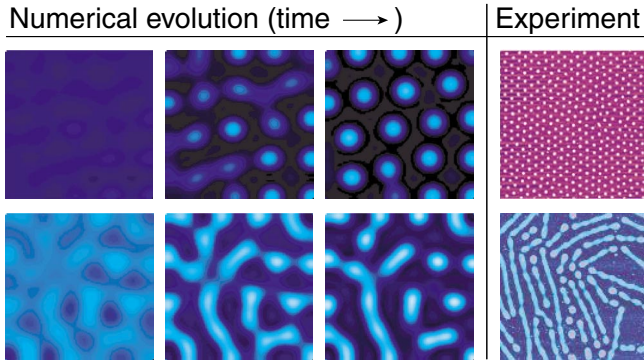
FIG. 2 (color online). Two numerical time series with different initial concentrations showing the evolution of dots and pearling compared with experimental (SFM) images. Dot diameters and stripe widths in the experimental images are both approximately 100 nm. Parameters in the numerical simulation correspond to a 51 k polymer with initial concentration c_0 = 0.84 \times 10^{10} molecules/cm 2 (top row) and c_0 = 3.3 \times 10^{10} molecules/cm 2 (bottom row). Black in the numerical data indicates a clean interface with no polymer, and light colors indicate high polymer concentrations. Both PS and PEO are concentrated within the dots and stripes.
